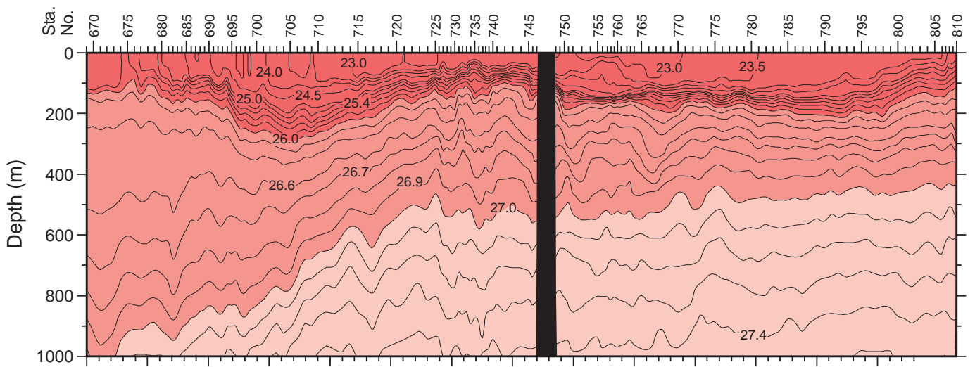
\sigma_0 (red), \sigma_2 (green), \sigma_4 (blue) ( \text{kg/m}^3 ) for I07 60°E
