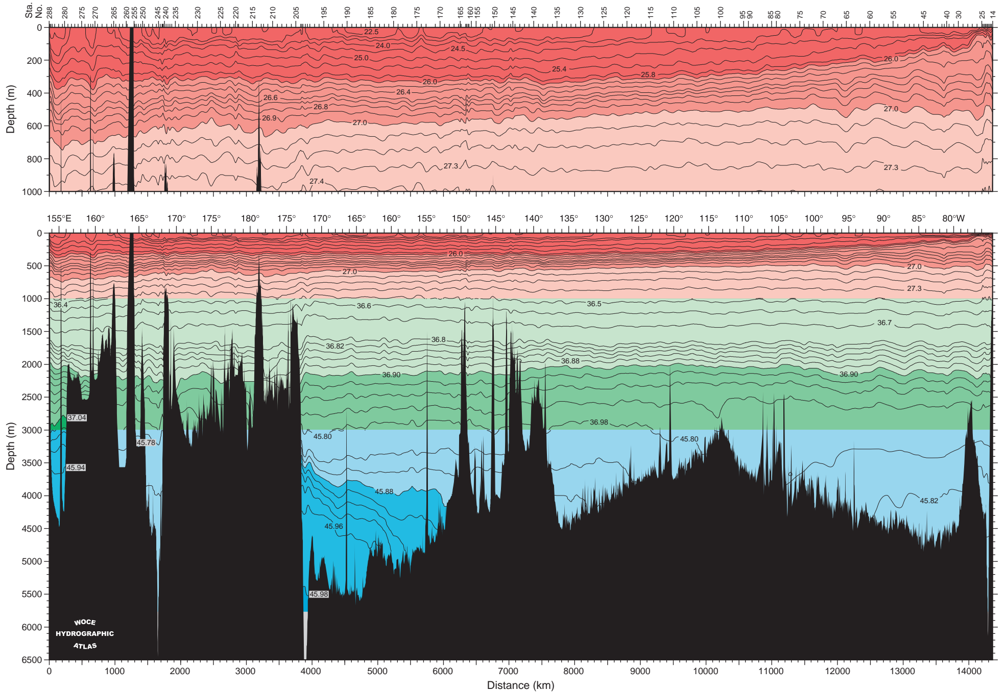
\sigma_0 (red), \sigma_2 (green), \sigma_4 (blue) for P21 17°S
