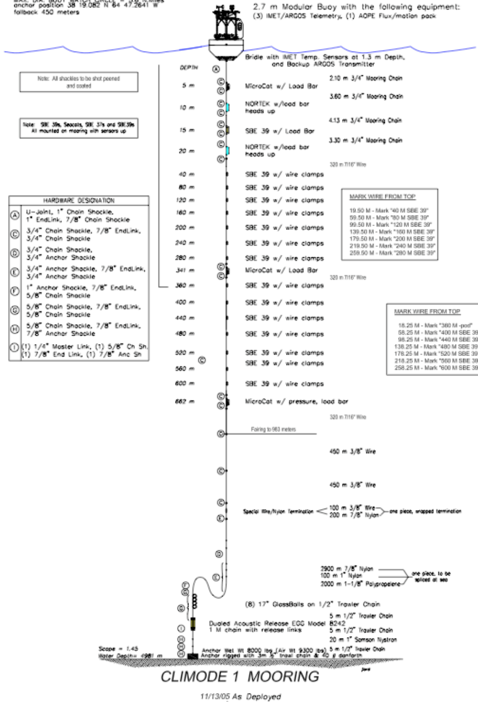
Figure 2: CLIMODE 1 Mooring F Diagram
