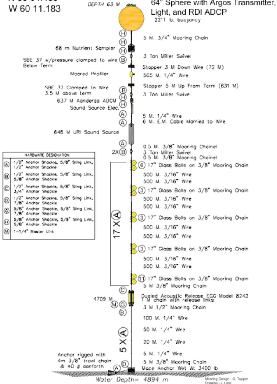
Figure 11. Subsurface Mooring D diagram.
